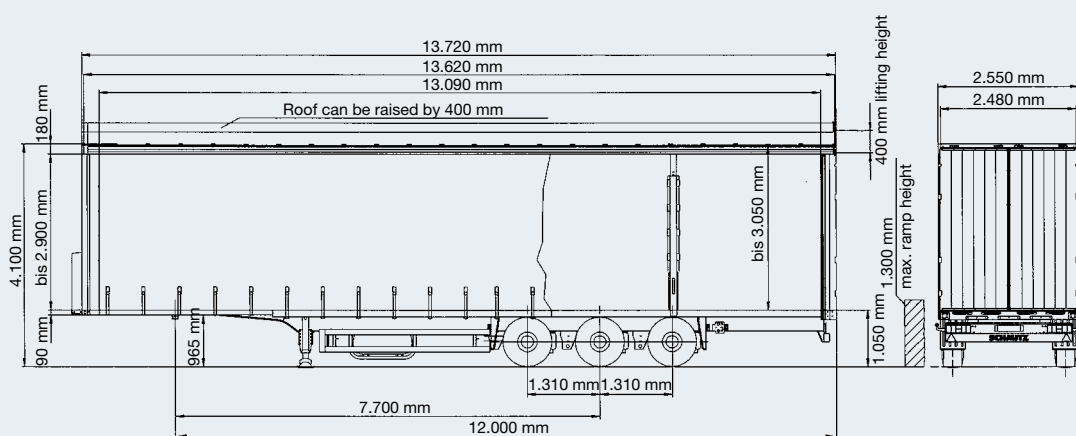
S.CS 24/L – 13.62 MB – VARIOS® – large volume carrying, three-axle semitrailer with curtainsider tensioned tarpaulin design
