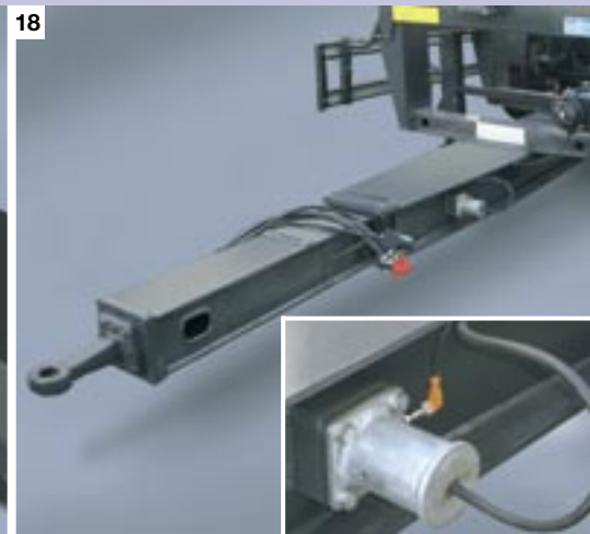
18. Telescopic tow bar (1 x 100 mm / 1 x 900 mm) with pneumatic locking.
