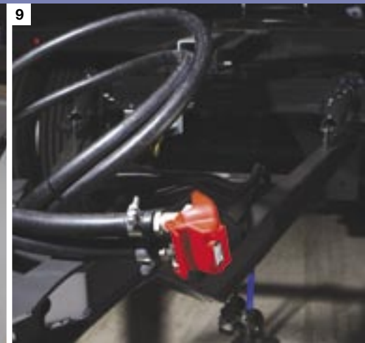
9. DUOMATIC air connection.
