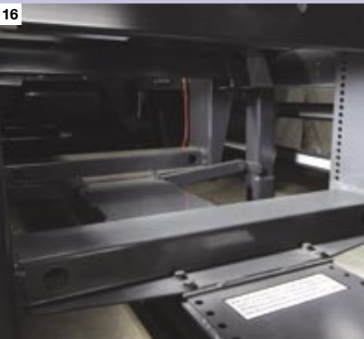
16. Length and height adjustable tow bar.
