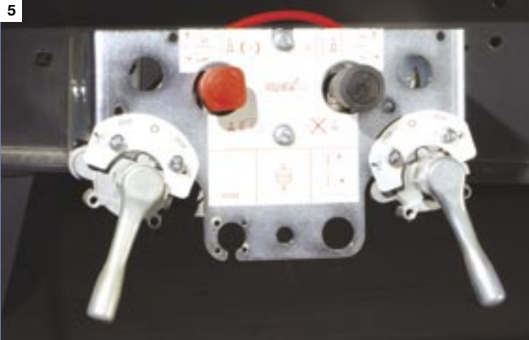
5. Control unit for park brake and air suspension with 2 lifting & lowering valves mounted on the side of the A.WF longitudinal member.
