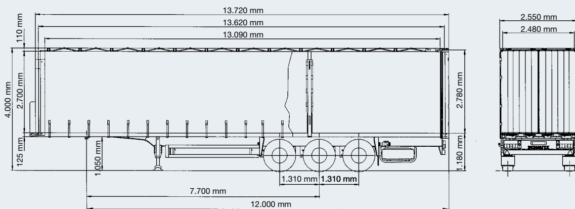
S.CS 24/L – 13.62 EB – three-axle semitrailer with curtainsider tensioned tarpaulin design
