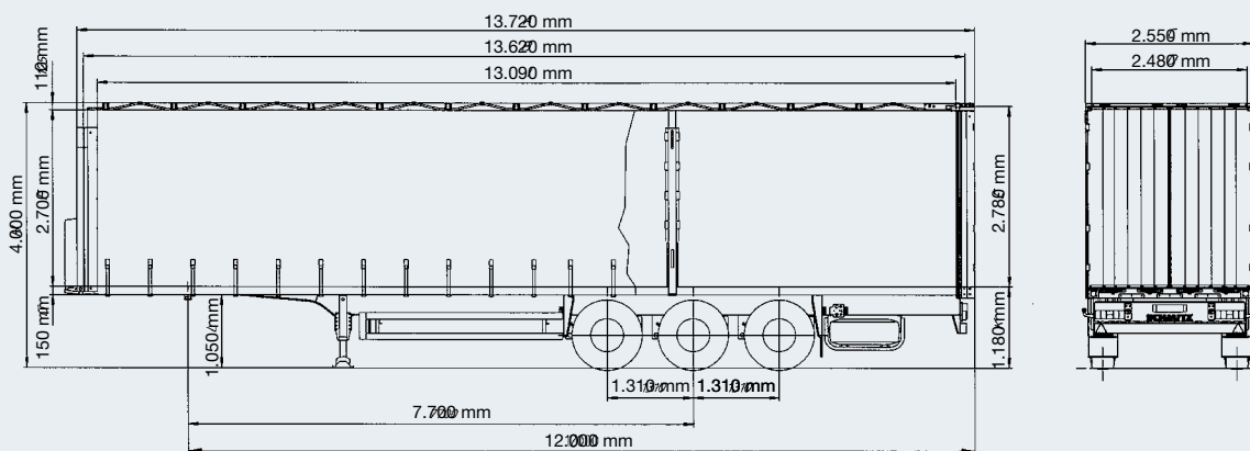
S.CS 24/L – 13.62 LB – three-axle semitrailer with curtainsider tensioned tarpaulin design
