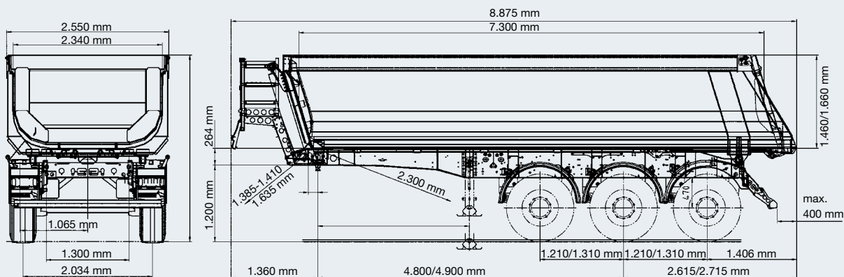
Three-axle rear tipper semitrailer design: steel body with chute and platform
