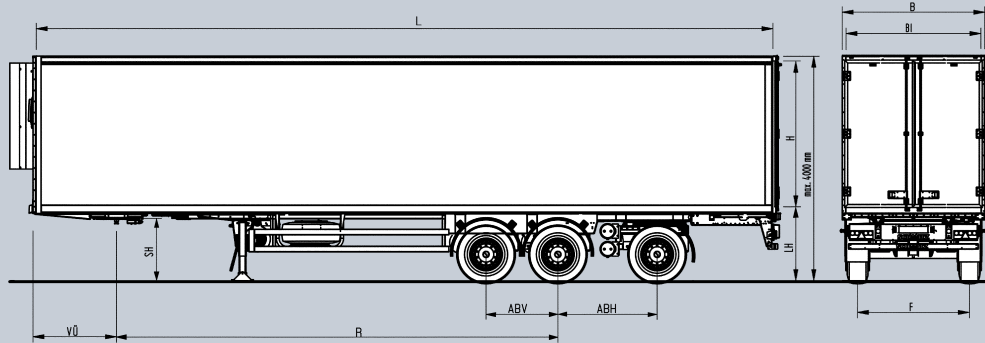
S.KO - 24/LZG Three-axle – Semitrailer – Force-steered
