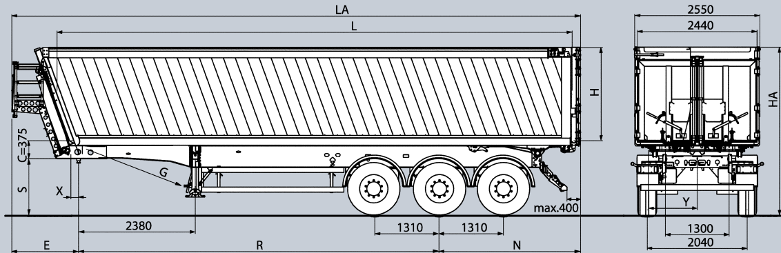
S.KI 24 / 10.5 SL06 AK Three-axle rear tipper semitrailer with aluminium box-body
