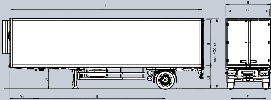
S.KO - 10/LZG Single-axle – Semitrailer – Force-steered
