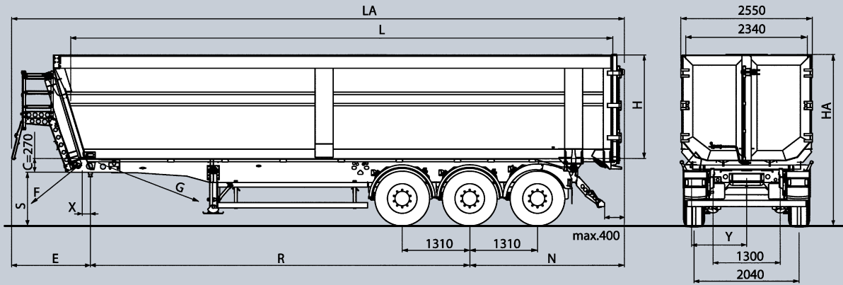
S.KI 24 / 10.5 SL06 SR Three-axle rear tipper semitrailer with rounded steel body
