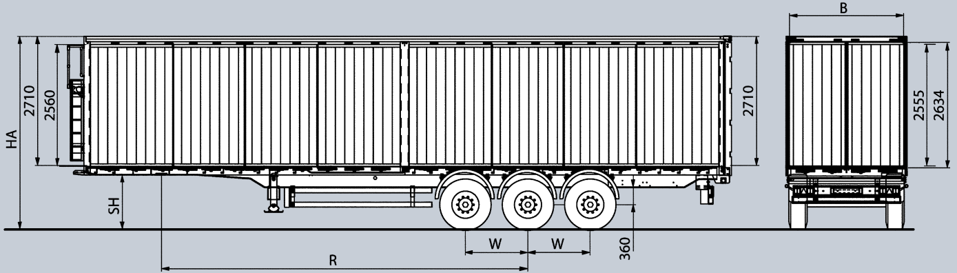
Three-axle rear semitrailer with sliding floor
